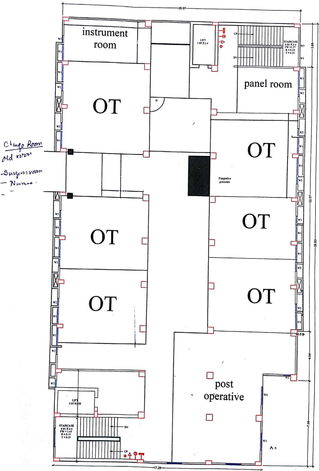
FIRST FLOOR PLAN (ANNEXE BLOCK)
